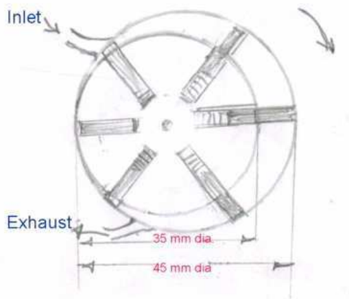
Fig. 1 Compressed Air Turbine –Concept & Cycle
