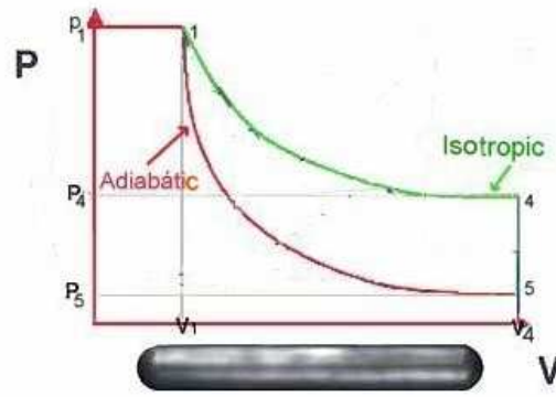
Fig.2 Isotropic cycle for Air Turbine
